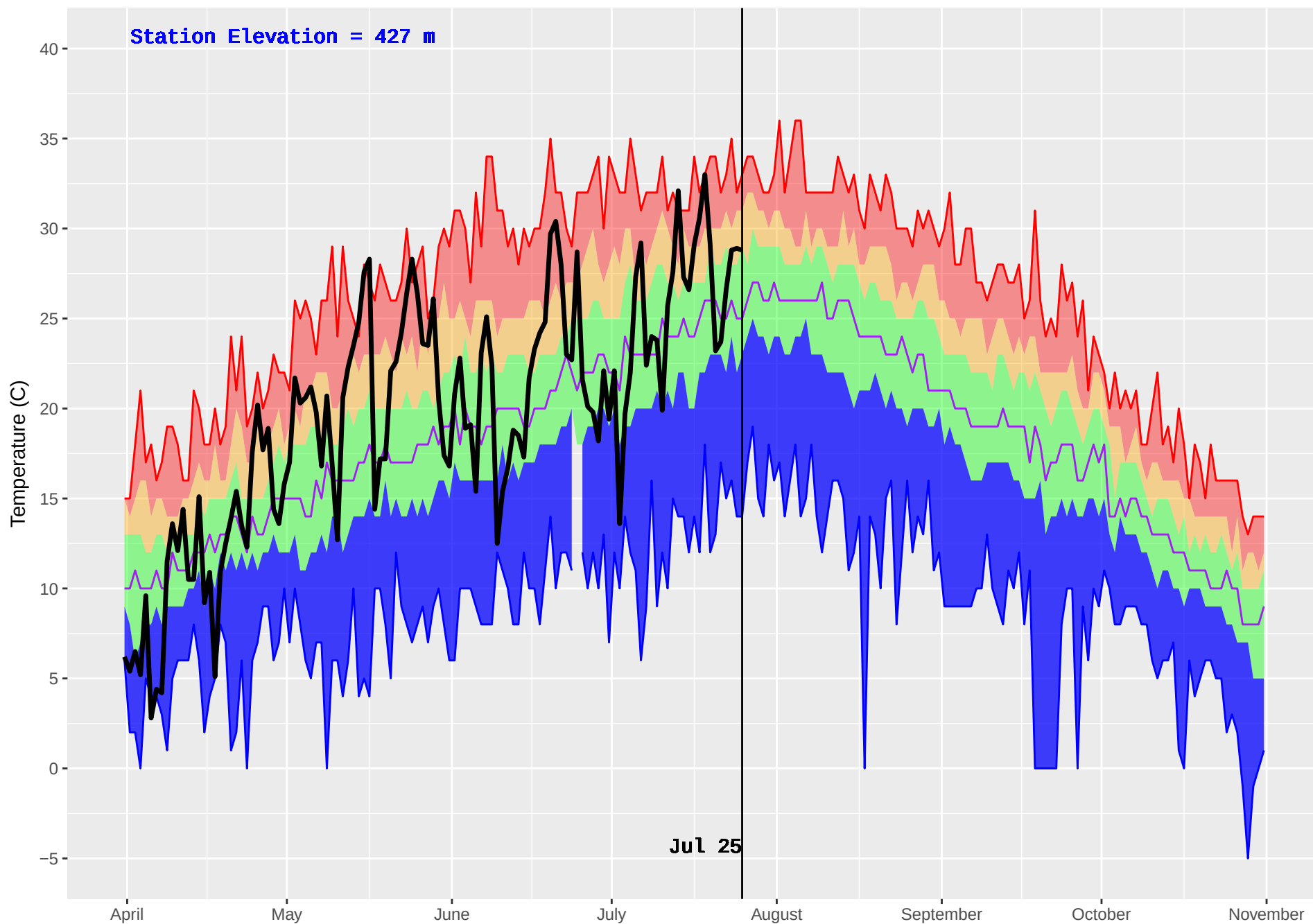
PENTICTON RS (328) : Historical (1970–2016) and Current (2018) Noon Temperature
