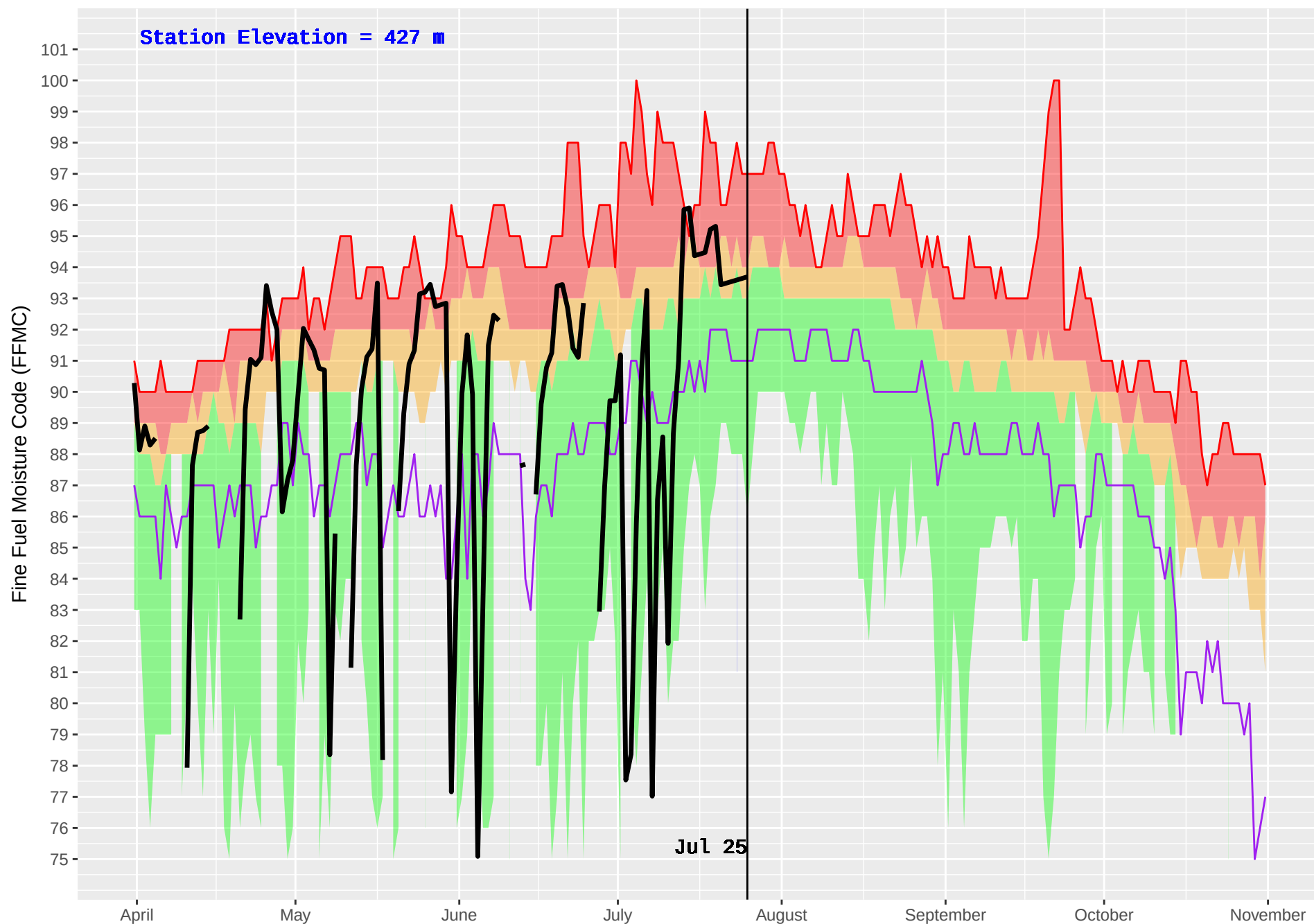
PENTICTON RS (328) : Historical (1970–2016) and Current (2018) Noon Fine Fuel Moisture Code (FFMC)
