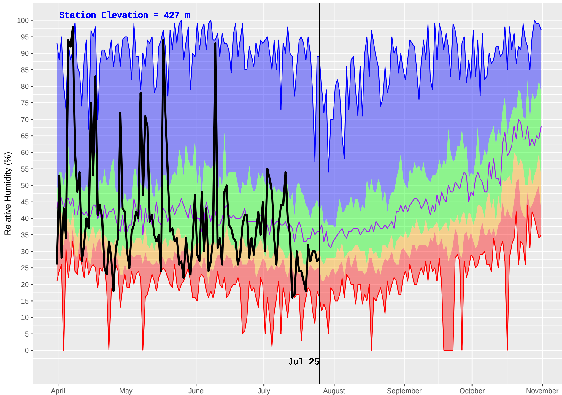
PENTICTON RS (328) : Historical (1970–2016) and Current (2018) Noon Relative Humidity
