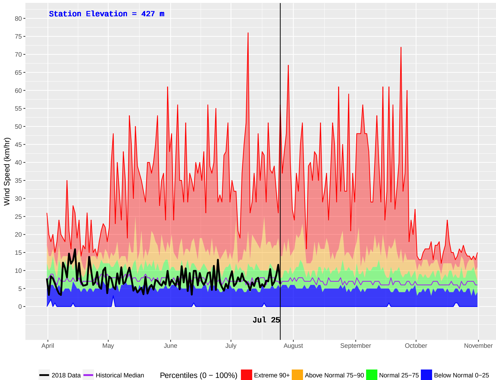
PENTICTON RS (328) : Historical (1970–2016) and Current (2018) Noon Wind Speed
