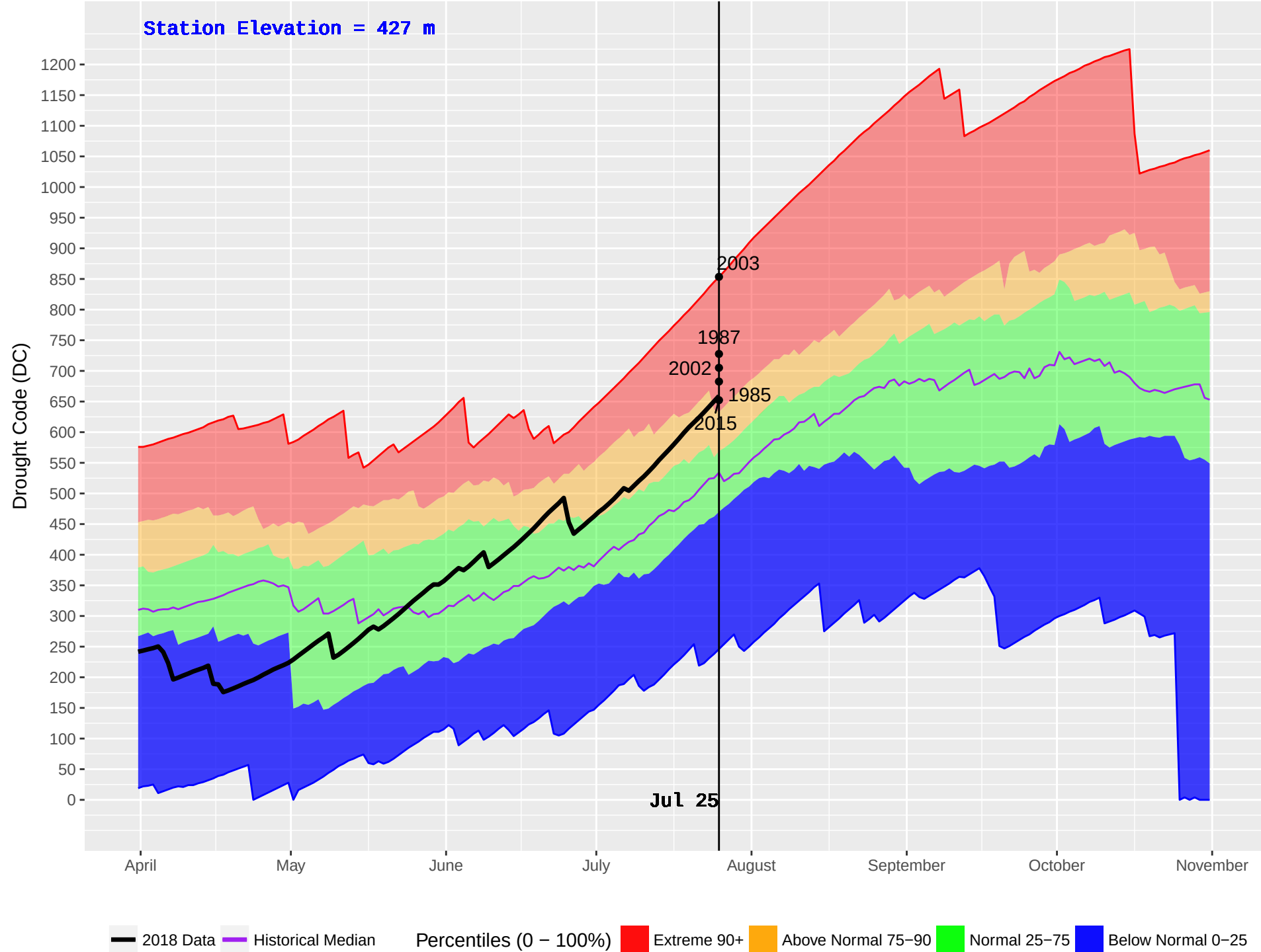
PENTICTON RS (328) : Historical (1970–2016) and Current (2018) Noon Drought Code (DC)
