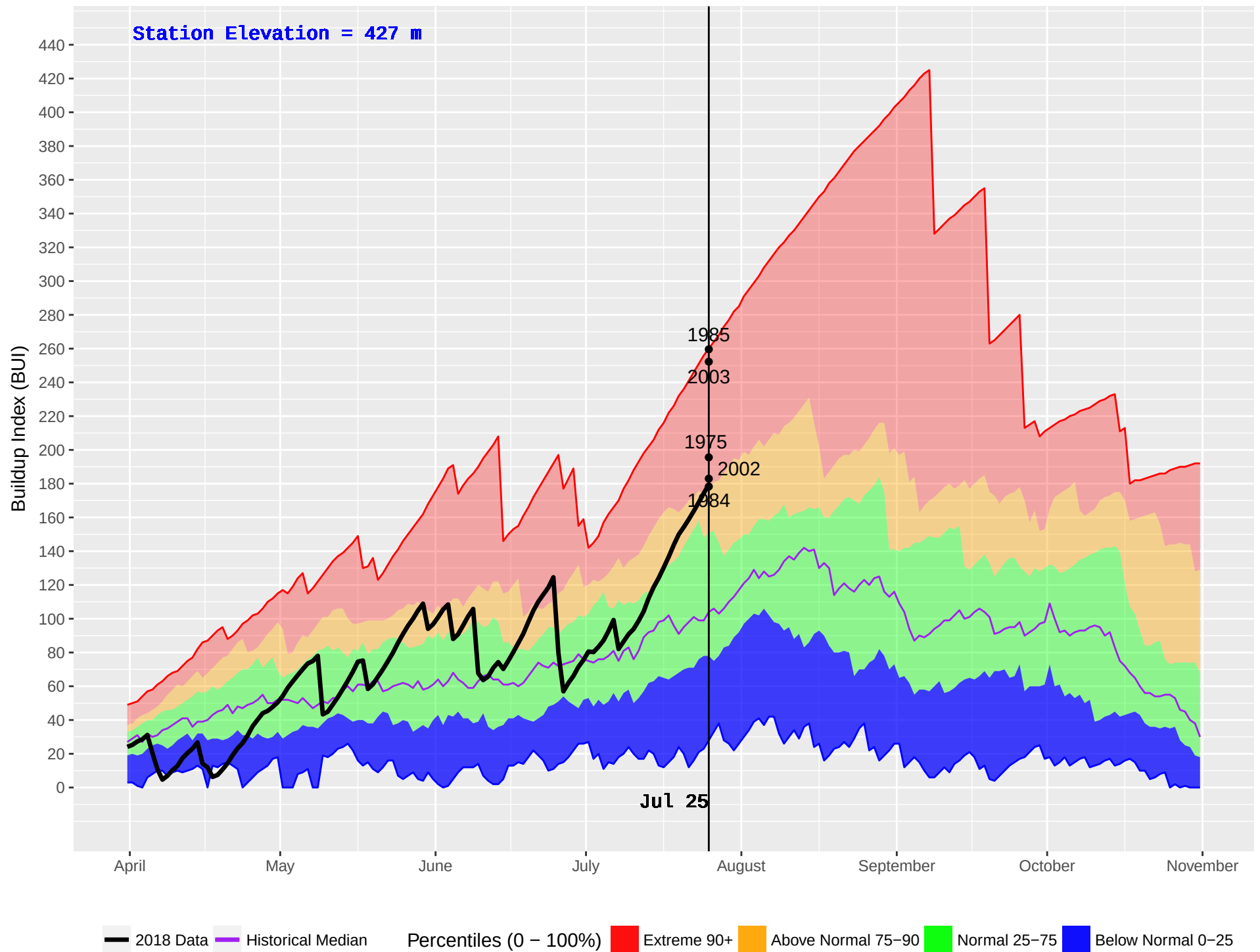
PENTICTON RS (328) : Historical (1970–2016) and Current (2018) Noon Buildup Index (BUI)
