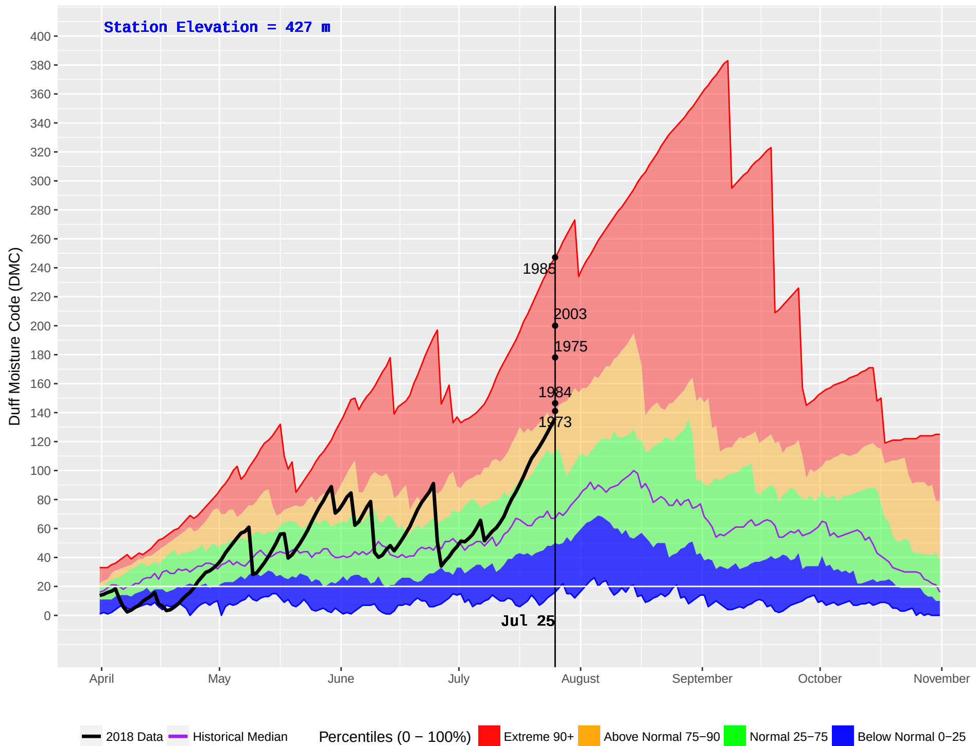
PENTICTON RS (328) : Historical (1970–2016) and Current (2018) Noon Duff Moisture Code (DMC)
