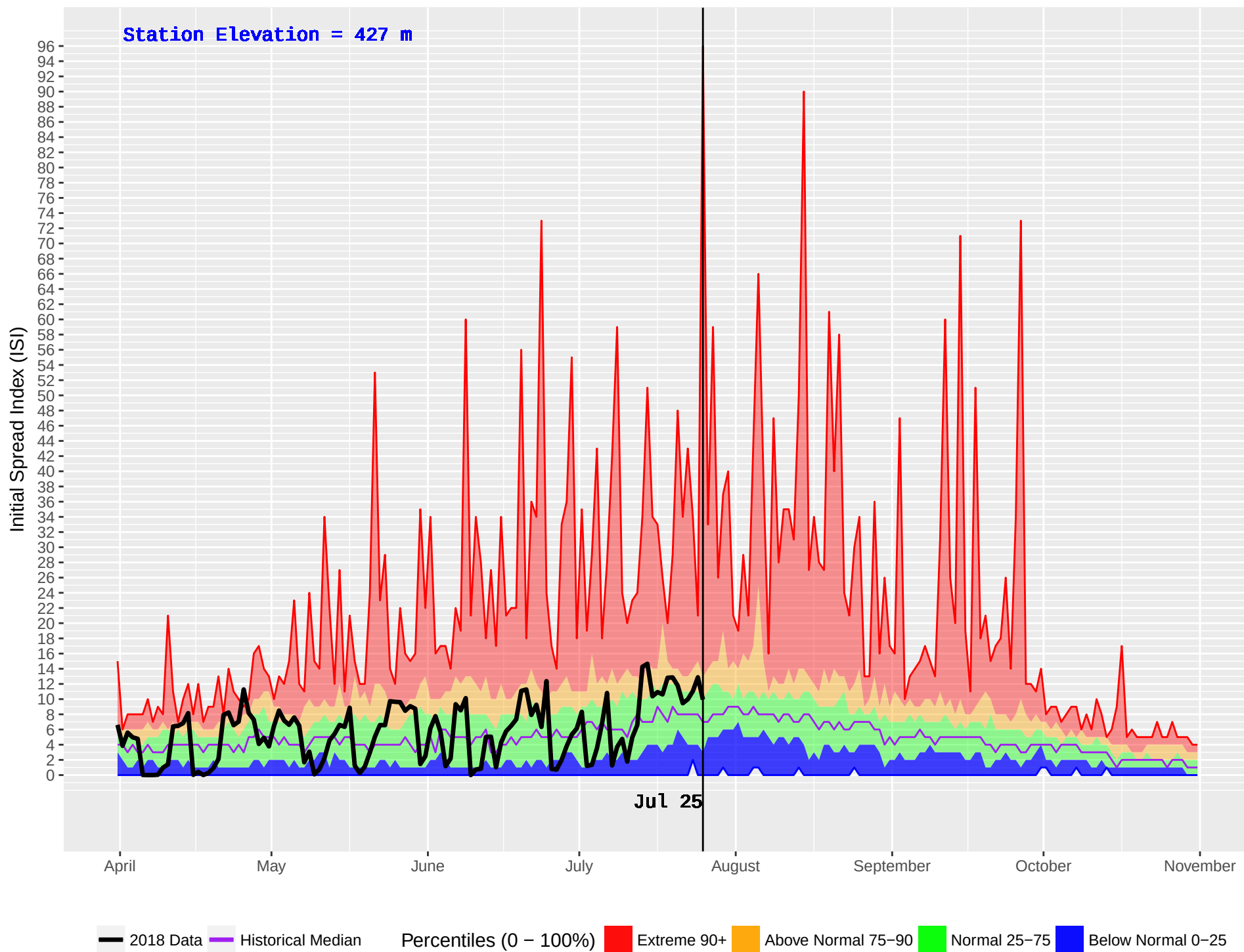
PENTICTON RS (328) : Historical (1970–2016) and Current (2018) Noon Initial Spread Index (ISI)
